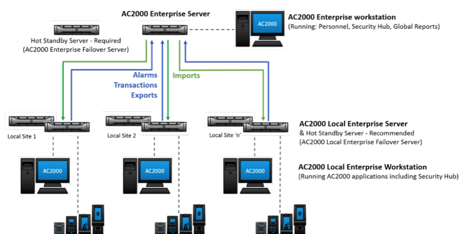
AC2000 Enterprise server and AC2000 Local Enterprise server information flow
